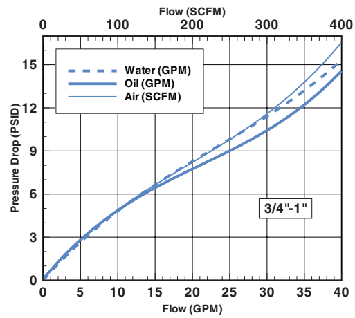
SERIES 4 -40 FLOW METER
