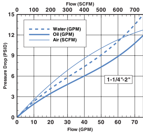
SERIES 5 -75 FLOW METER
