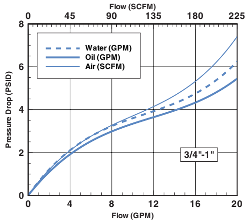
SERIES 4 -20 FLOW METER
