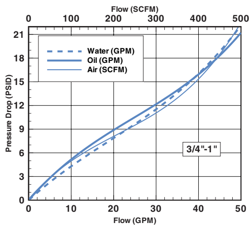
SERIES 4 -50 FLOW METER
