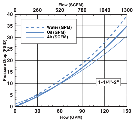
SERIES 5 -99 FLOW METER
