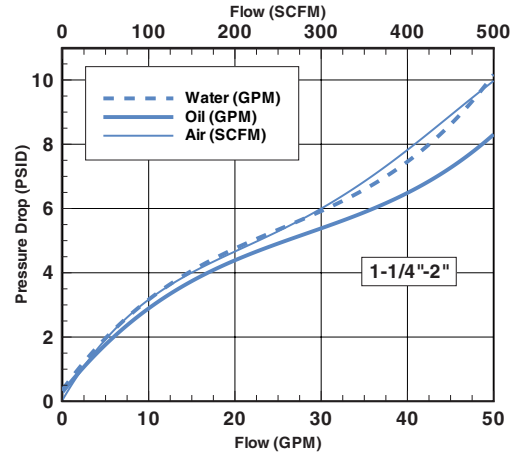
SERIES 5 -50 FLOW METER
