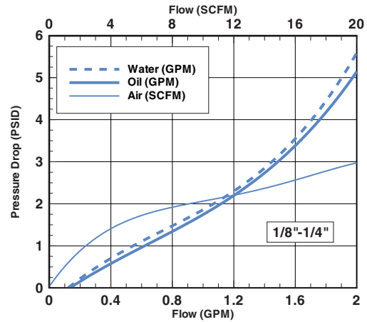
SERIES 2 -02 FLOW METER
