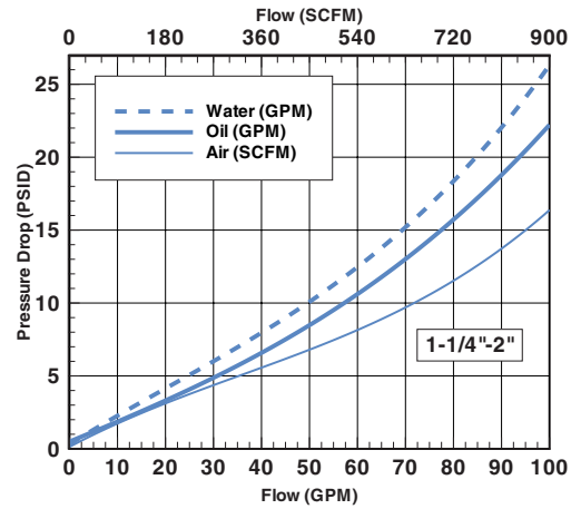
SERIES 5 -88 FLOW METER
