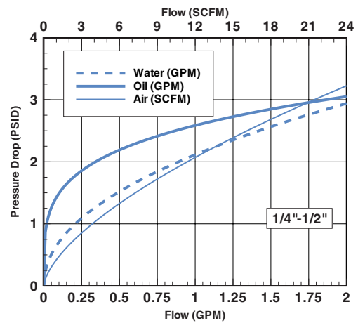
SERIES 3 -02 FLOW METER
