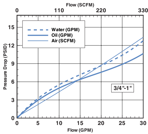
SERIES 4 -30 FLOW METER
