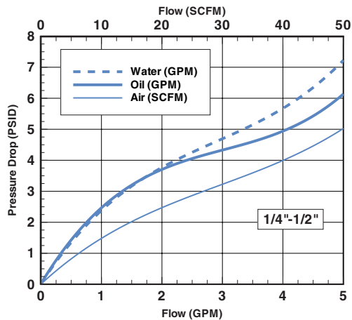
SERIES 3 -05 FLOW METER
