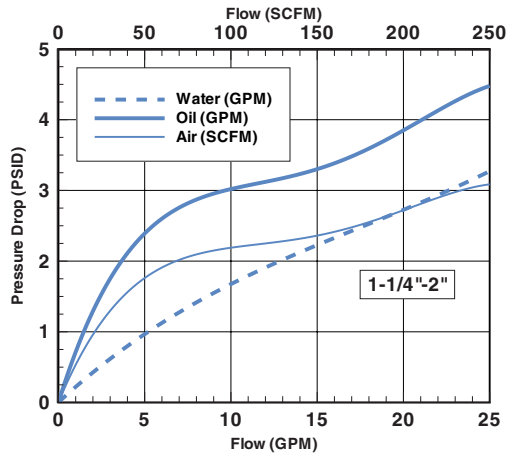
SERIES 5 -25 FLOW METER
