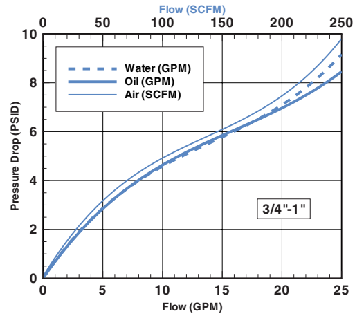
SERIES 4 -25 FLOW METER
