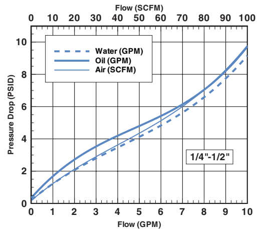
SERIES 3 -10 FLOW METER
