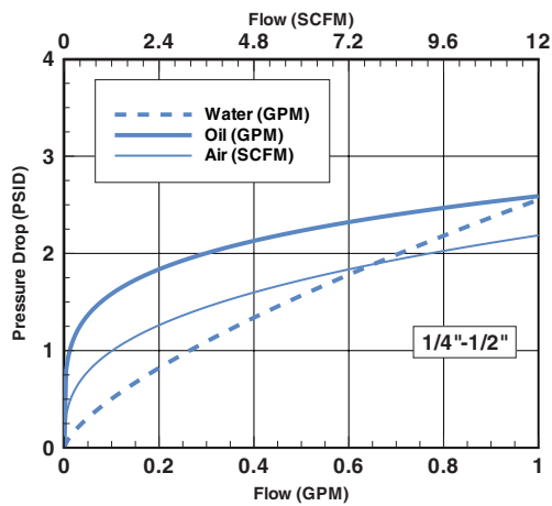
SERIES 3 -01 FLOW METER
