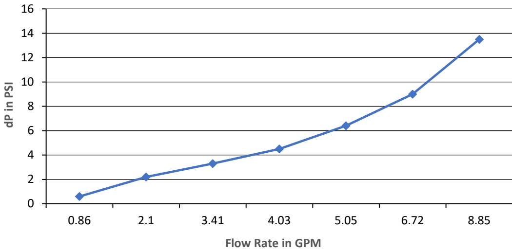
TRG-11.500-5 Pressure Drop (1.5cst)
